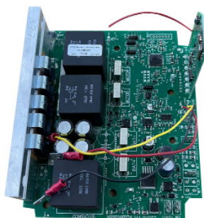
DC AUTO STOP CIRCUIT BOARD PART #BOARD, DC AUTO STOP Replacement circuit board for DC Autostop Motor only. Board uses wireless remotes and Bluetooth. Also allows you to set upper and lower limits. Will only work with the blue remotes. Multiple safety features are built into the circuit board.
